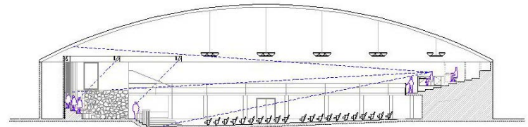
BUILDING LONGITUDINAL SECTION
